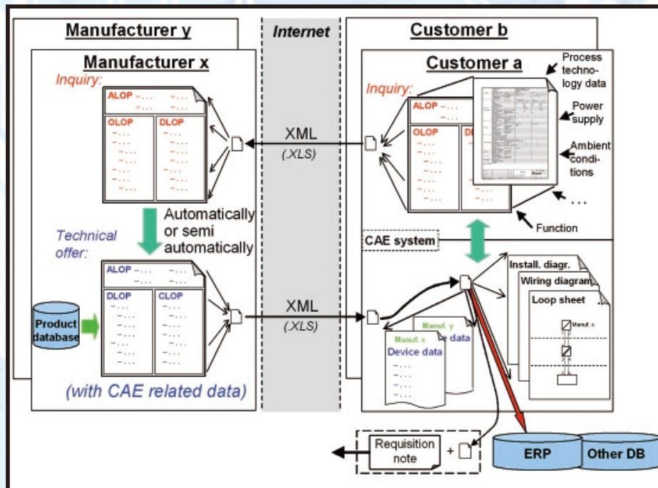
Figure 7: Data exchange in the engineering workflow between customer and manufacturer
