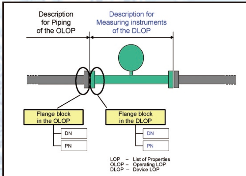
Figure 5: Interrelationship between properties in the OLOP and DLOP
