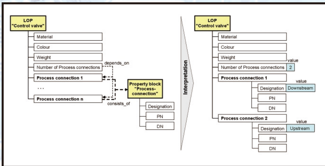
Figure 3: Example of block structure and cardinality, illustrated by part of an LOP.
