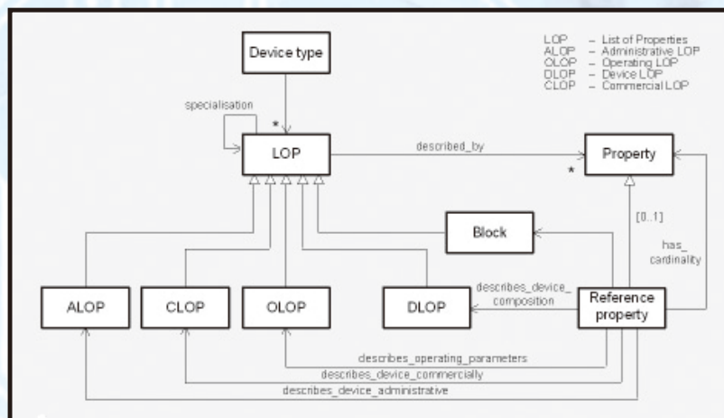
Figure 4: Simplified UML schema of an LOP
